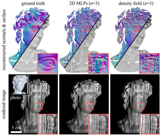
Figure 4: MLPs and density fields for inverse SL. Reconstructing a statue from n = 3 SL images using a la carte projection patterns of maximum frequency 128 [31]. The MLP-based reconstruction has many artifacts and does not reproduce the input images. While the volumetric approach reproduces the images faithfully, the recovered surface is inaccurate.
