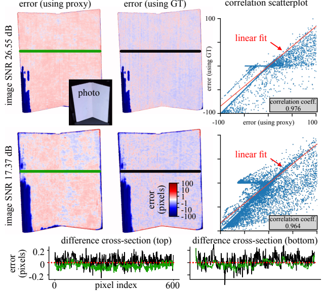
Figure 6: No-reference proxy for disparity error. Comparison of the signed difference between front-to-back and back-to-front disparity maps (left) and between front-to-back and ground-truth maps (middle) for a wedge-like surface reconstructed from two sets of SL images—one captured (top) and one with extra 1% Gaussian noise added to the captured set (bottom). The difference cross-sections show agreement to within a fraction of a pixel, and the scatter-plots demonstrate strong correlation across all disparity errors. The SL patterns used were the same as in Figure 4.
