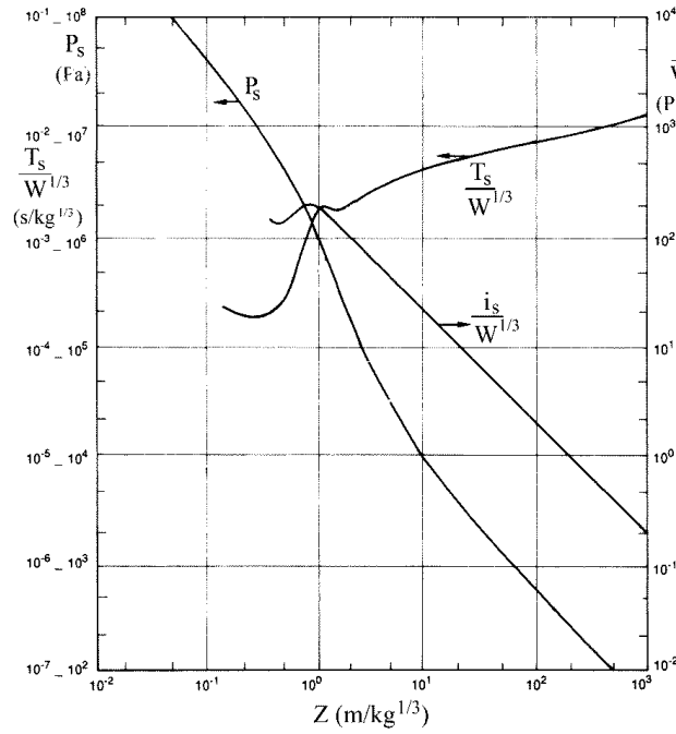
Figure 3: The blast curves for static overpressure ( P_s ) and scaled pulse period ( \frac{T_s}{W^{1/3}} ) as a function of scaled distance Z (from [19]). These curves are for spherical TNT charges, exploded in air, at ambient conditions.
