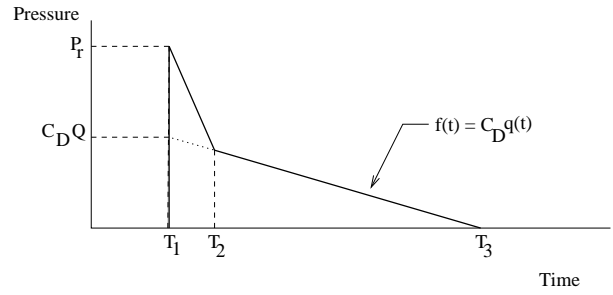
Figure 6: Translatory Pressure versus Time.
